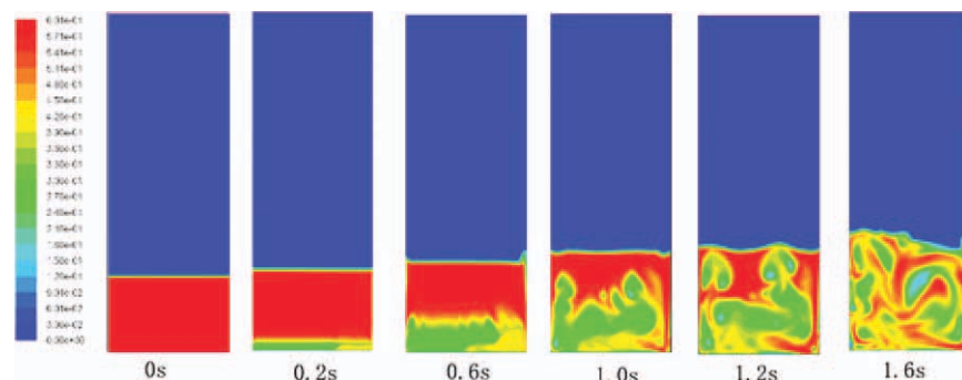
Figure 14. The evolution of solid volume fraction contour in the reactor in Case 5.
