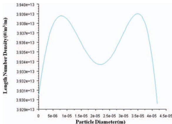
Figure 8. The length number density of initial particles in Case 1.
